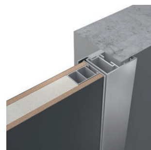
U-SYSTEM frame Installation in an finished opening
